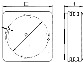
INSTAT 868-a1A, INSTAT 868-a1mA t = 27,8 mm; □ = 75 mm INSTAT 868-a1T t = 26,8 mm; □ = 71 mm
